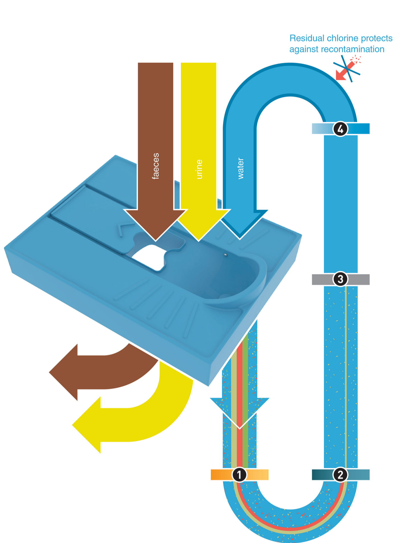
Schematic of the multi-barrier treatment for safe water recovery
