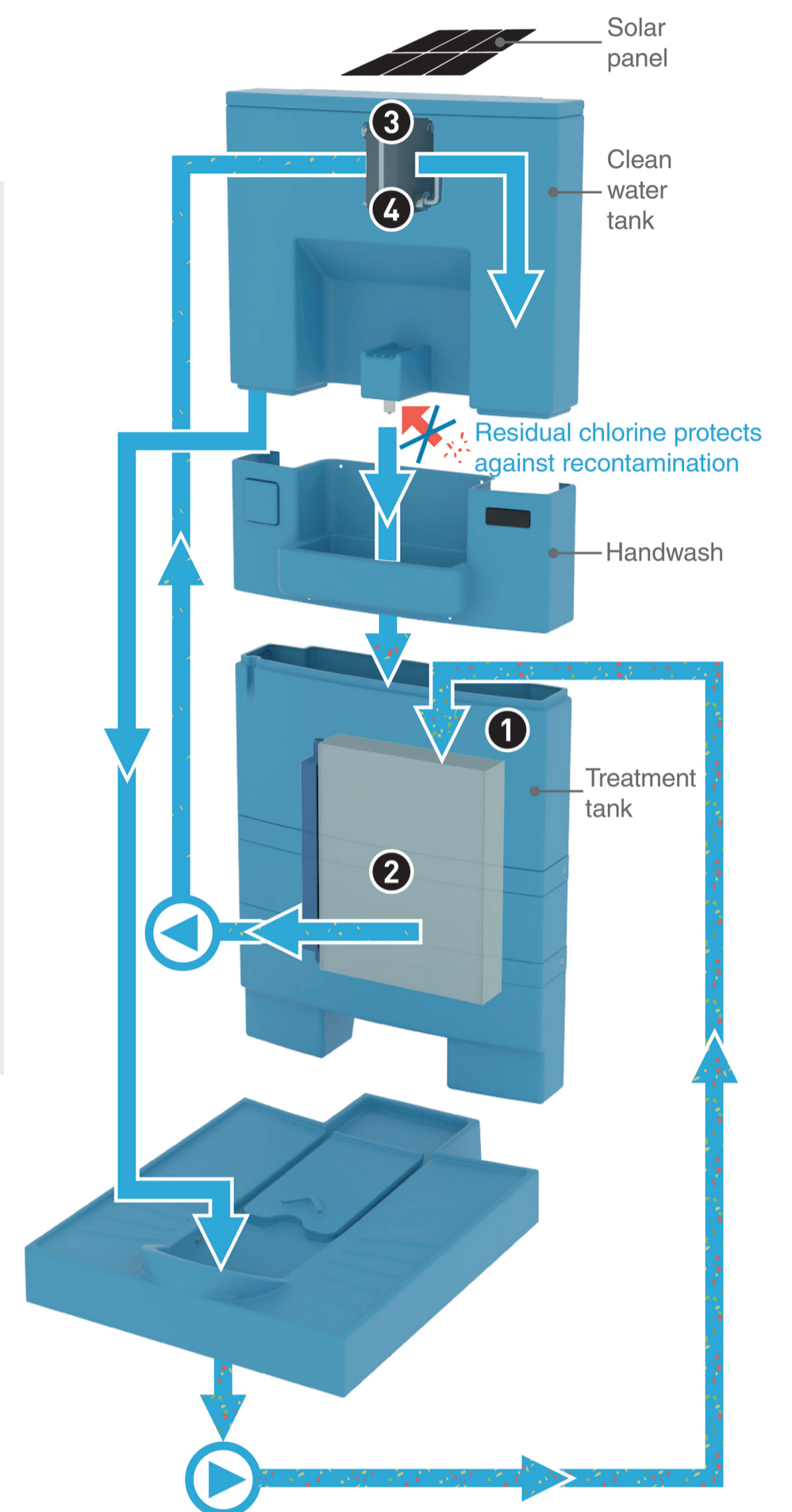
The water recovery technology inside the toilet
